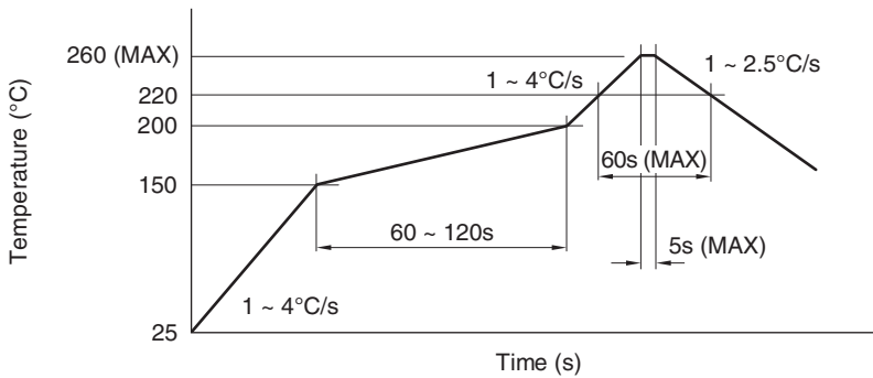
Fig. 18 Temperature Profile
