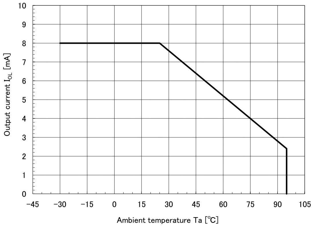
Fig.1 Output current vs. ambient temperature
