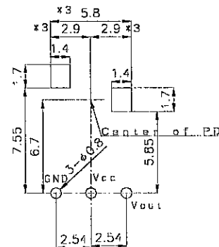
Example of mounting drawing from solder side(Reference)
