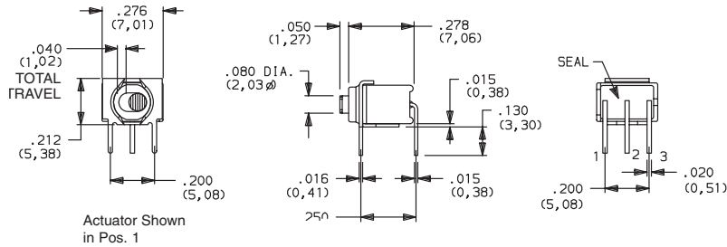
PC MOUNTING
