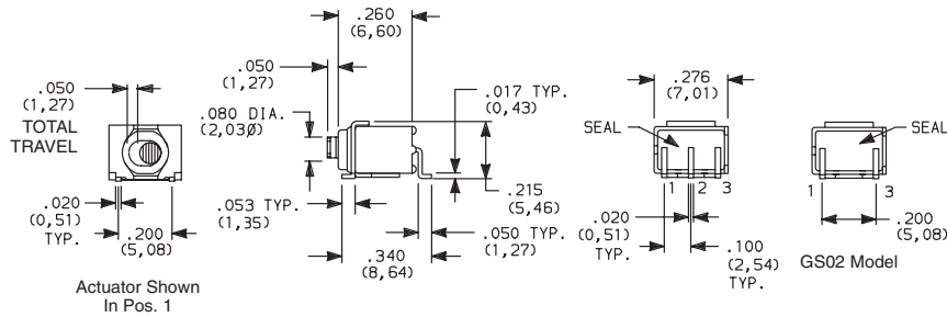
PC MOUNTING
