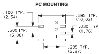
PC MOUNTING
