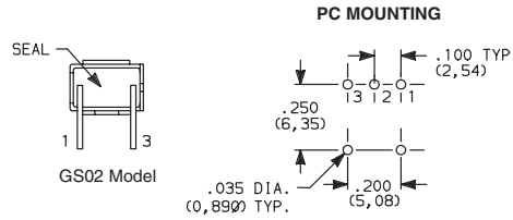
PC MOUNTING
