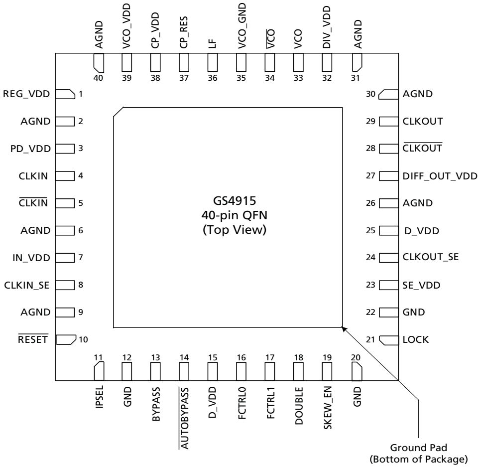
Figure 1-1: 40-Pin QFN
