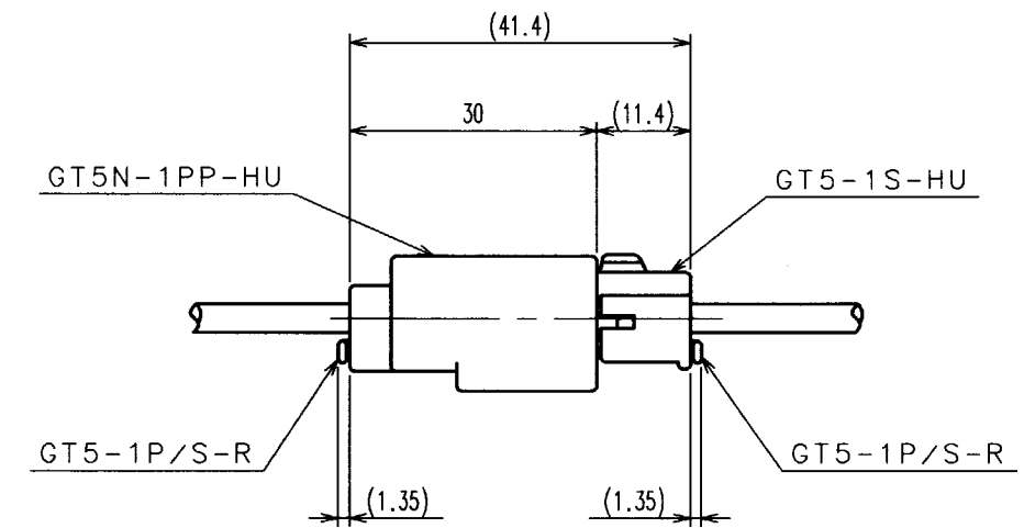
MATED CONNECTORS
