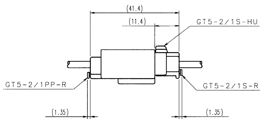
MATED CONNECTORS
