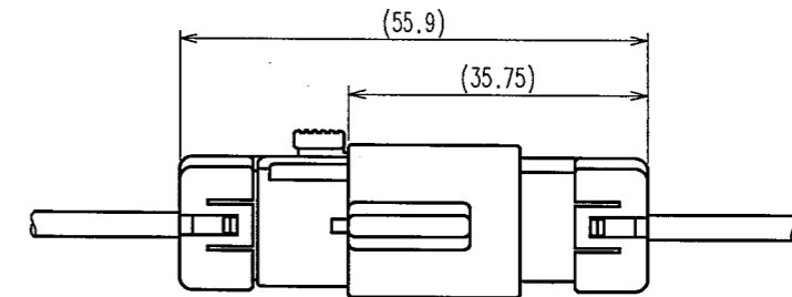
MATED CONNECTORS
