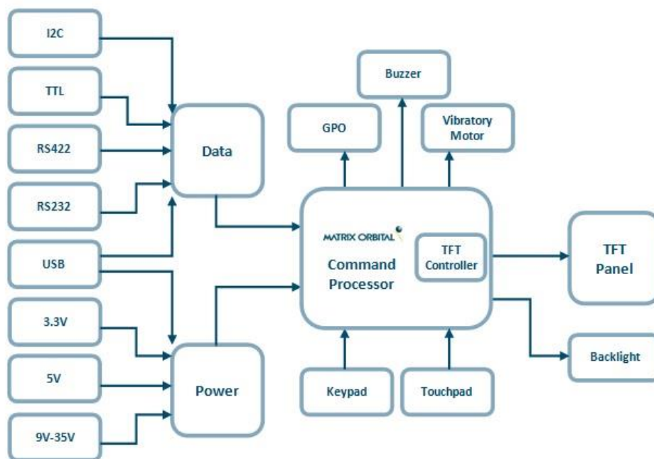
Figure 2: Functional Diagram
