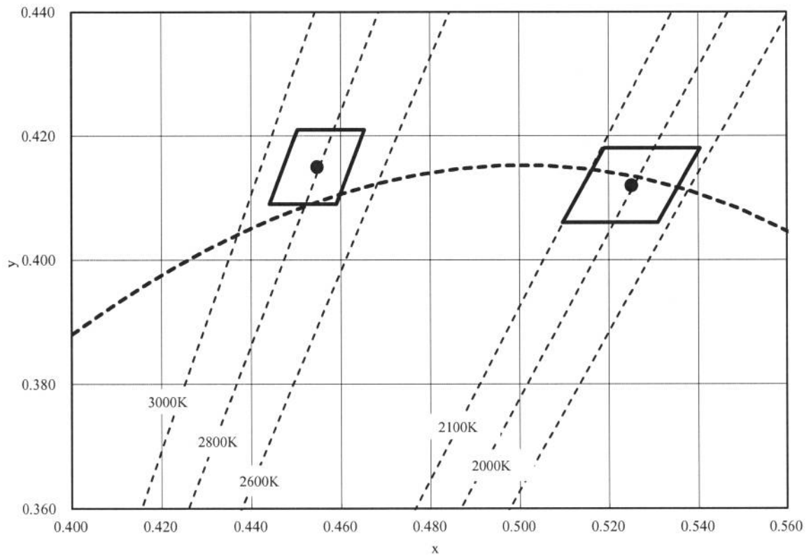
Chromaticity Diagram
