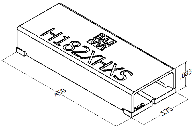
Isometric View
