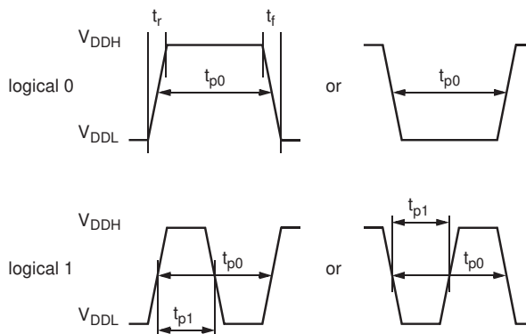
Fig. 5–1: Definition of logical 0 and 1 bit
