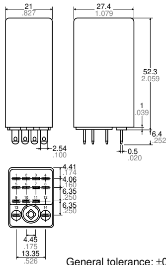
4 Form C External dimensions
