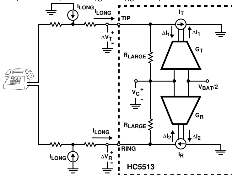
FIGURE 20A. FIGURE 20. LONGITUDINAL IMPEDANCE NETWORK
