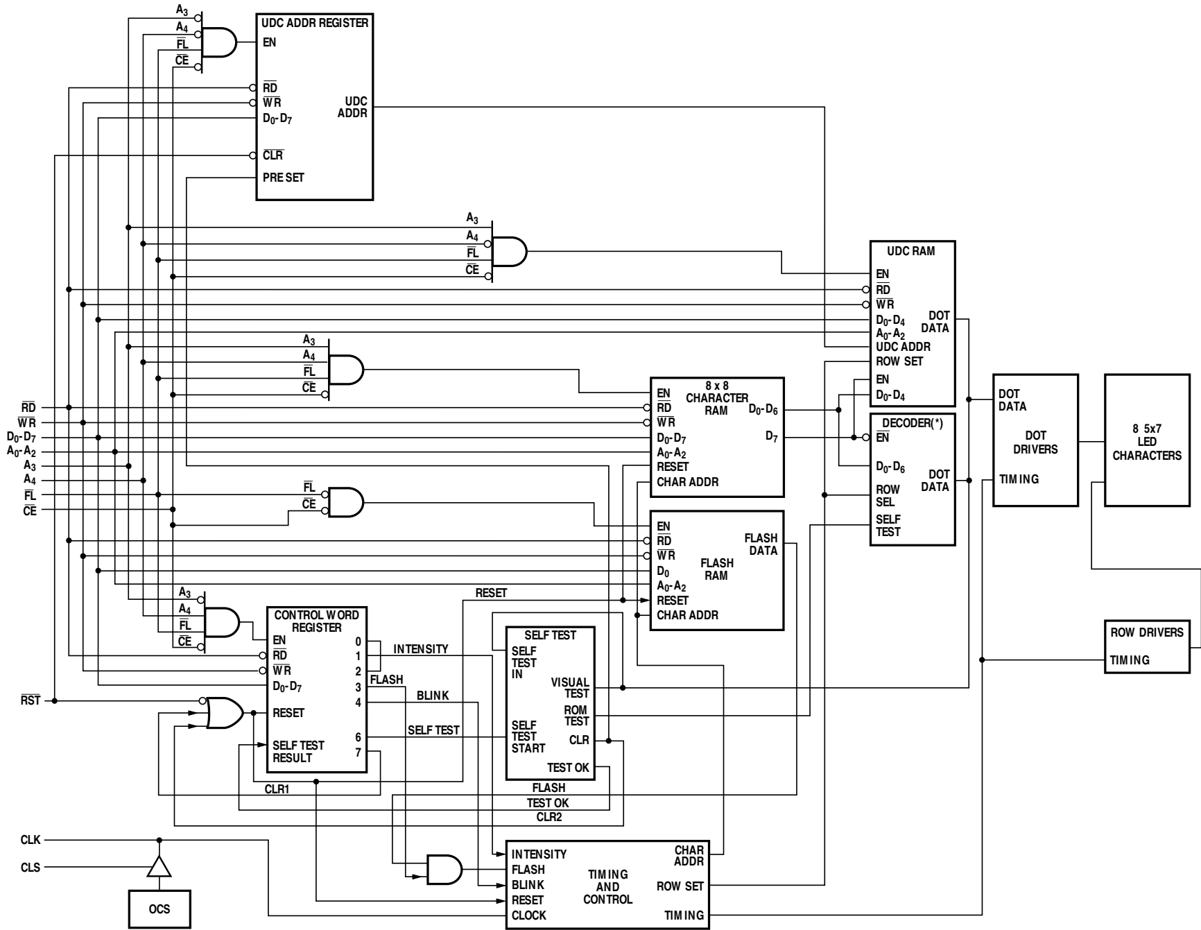
Figure 1. HDSP-213x/ -2179 internal block diagram.
