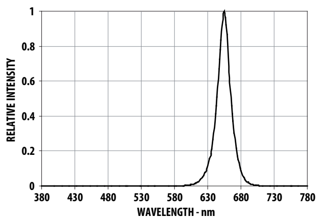
Figure 20. Relative Luminous Intensity Vs Wavelength
