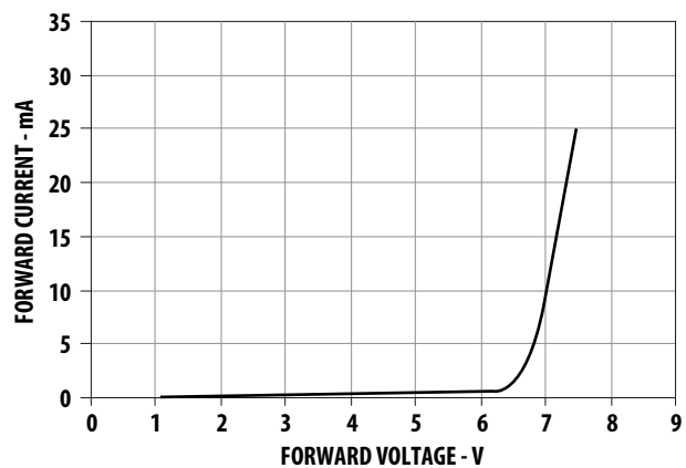
Figure 18. Forward Voltage Vs Current (Segment)
