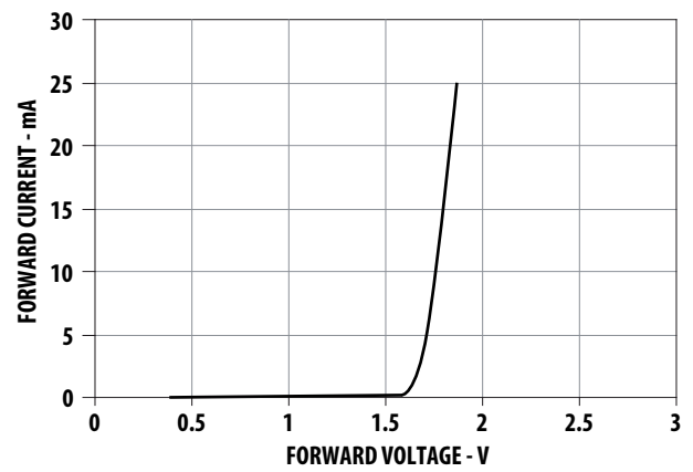
Figure 14. Forward Voltage Vs Current
