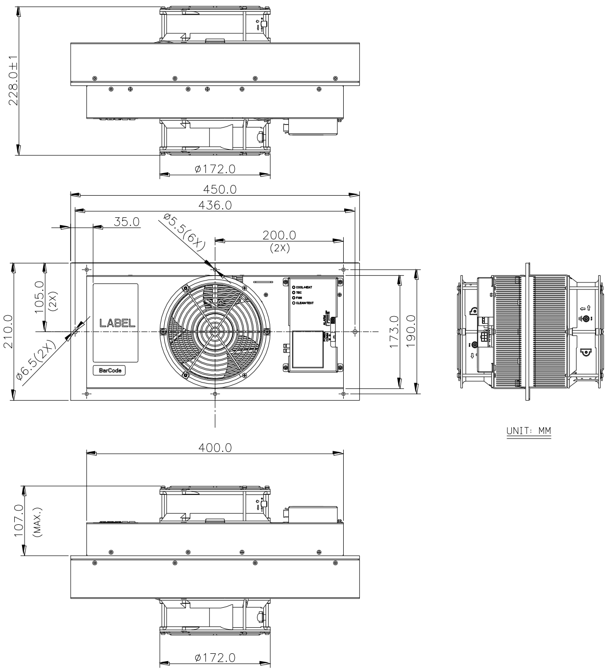
Dimension drawing
