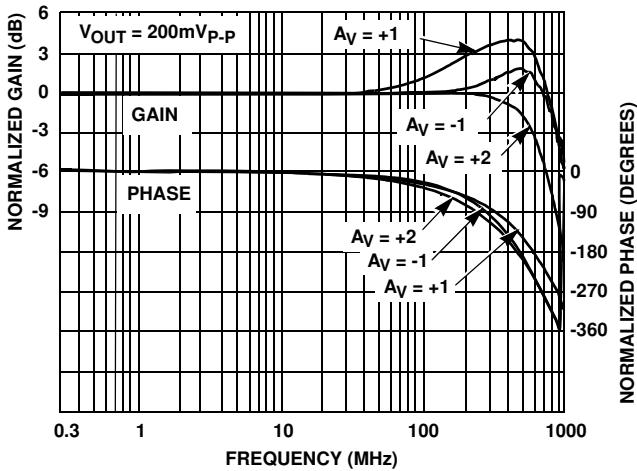
FIGURE 9. FREQUENCY RESPONSE
