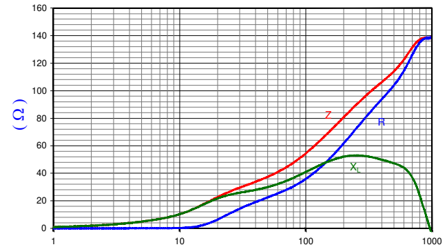
NET Z,R AND X vs. FREQUENCY (REF. ONLY)
