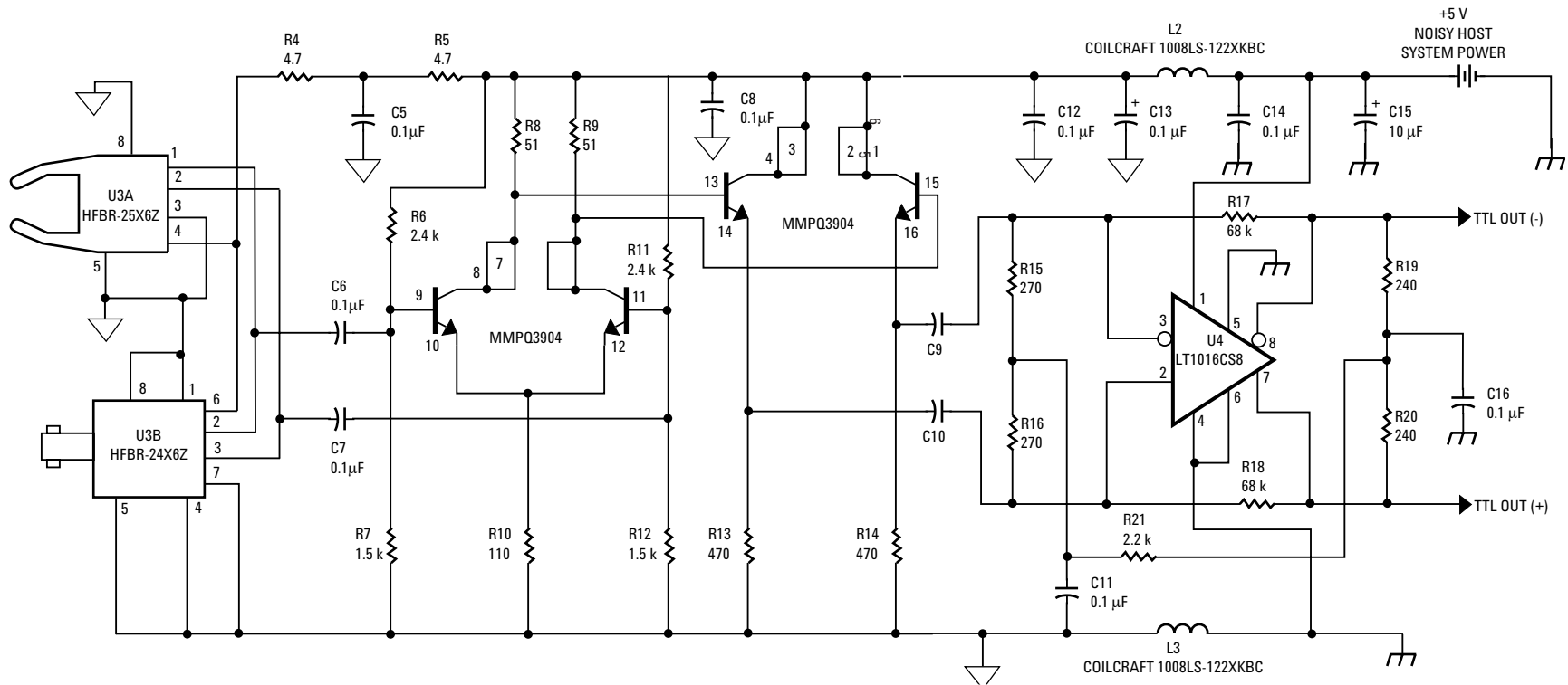
Figure 5. Enhanced Fiberoptic Receiver for use with dc to 32 MBd Arbitrary Duty Factor Data
