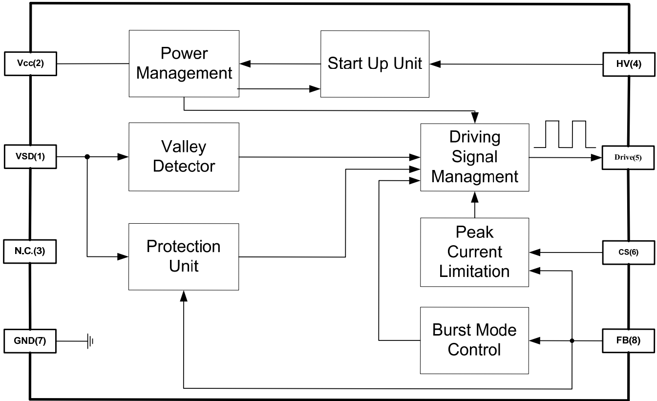
Figure 1— Block Diagram
