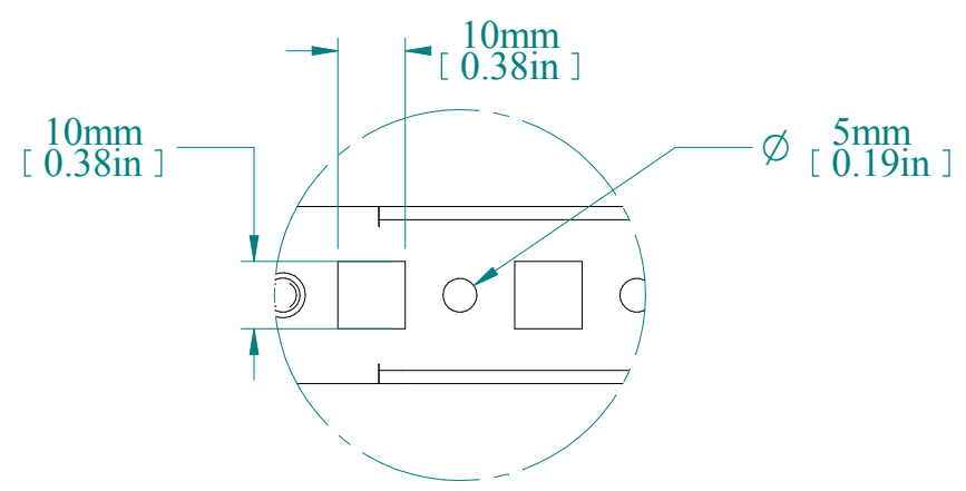
DETAIL A
