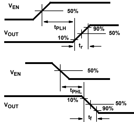
SWITCHING WAVEFORMS
