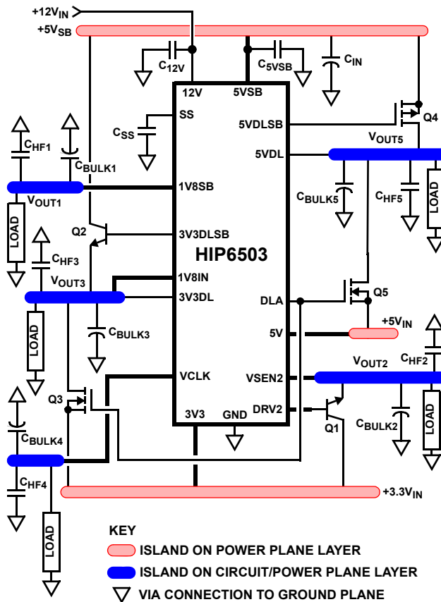
FIGURE 10. PRINTED CIRCUIT BOARD ISLANDS
