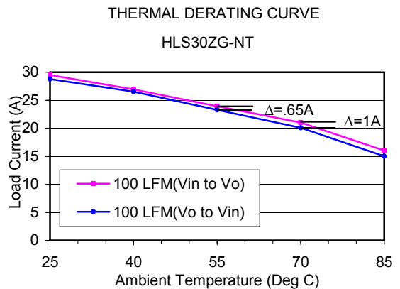
Figure 15. Effect of Airflow Direction on Power Rating [HLS30ZG (5V) shown]
