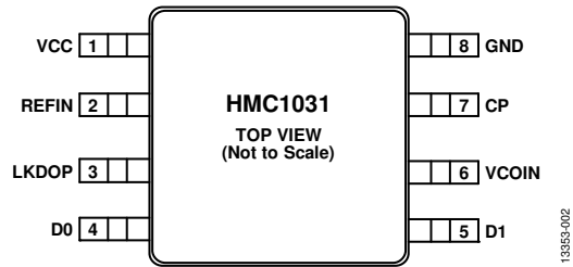
Figure 2. Pin Configuration
