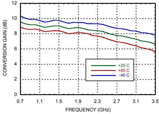
Conversion Gain vs. Temperature @ VGATE = 4.6V
