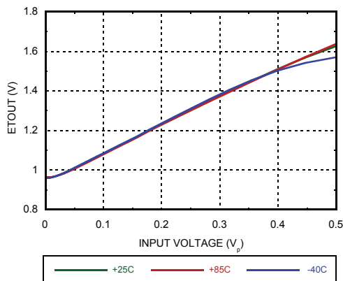
ETOUT vs. Vin with CW @ 1900 MHz
