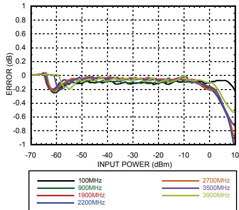
Reading Error for LTE 20MHz wrt CW Response @ -40 °C [1]
