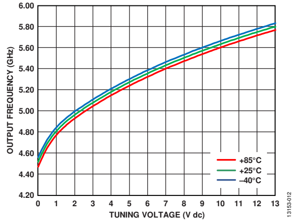
Figure 12. RFOUT/2 Output Frequency vs. Tuning Voltage ( V_{TUNE} )
