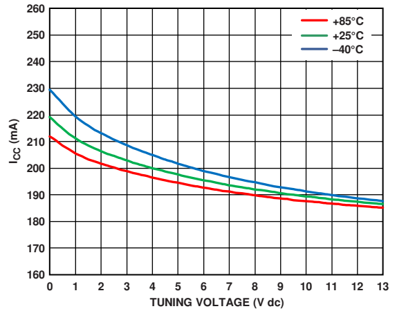
Figure 11. Supply Current ( I_{CC} ) vs. Tuning Voltage ( V_{TUNE} )
