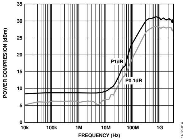
Figure 10. Input 1 dB Power Compression (P1dB) and Input 0.1dB Power Compression (P0.1dB) vs. Frequency, V_{CTL} = 0 V/5 V
