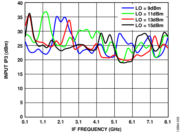
Figure 35. Input IP3 vs. IF Frequency at Various LO Power Levels, TA = 25°C
