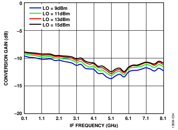
Figure 34. Conversion Gain vs. IF Frequency at Various LO Power Levels, TA = 25°C
