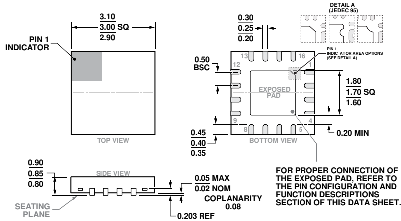
Figure 10. 16-Lead Lead Frame Chip Scale Package [LFCSP] 3 mm x 3 mm Body and 0.85 mm Package Height (CP-16-51) Dimensions shown in millimeters
