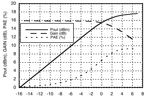
Power Compression @ 18 GHz
