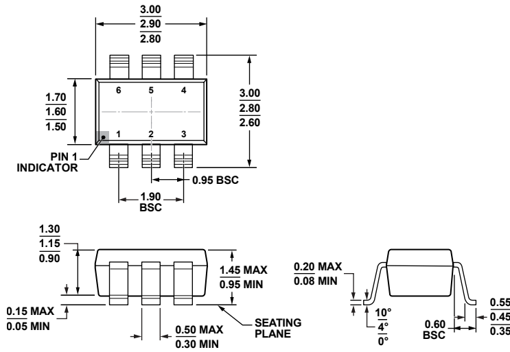
COMPLIANT TO JEDEC STANDARDS MO-178-AB Figure 13. 6-Lead Small Outline Transistor Package [SOT-23] (RJ-6) Dimensions shown in millimeters
