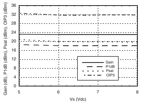
Gain, Power & OIP3 vs. Supply Voltage for Constant Icc= 62 mA @ 850 MHz
