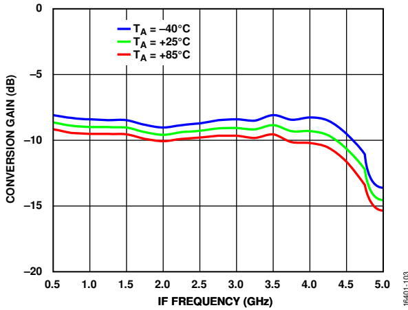
Figure 95. Conversion Gain vs. IF Frequency at Various Temperatures, LO = 15 dBm
