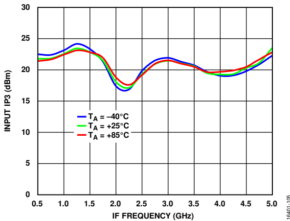
Figure 97. Input IP3 vs. IF Frequency at Various Temperatures, LO = 15 dBm
