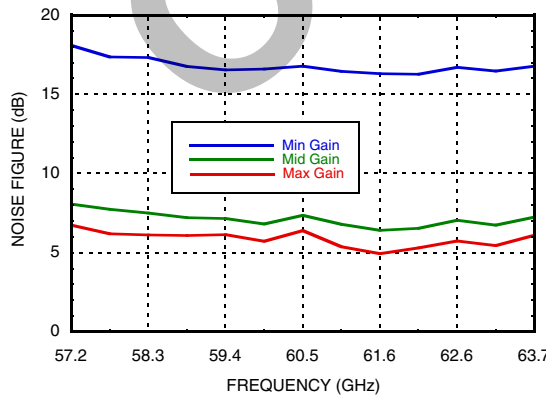
Figure 5. IC Noise Figure vs. Frequency and IF Gain [3]
