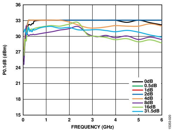
Figure 20. Input P0.1dB vs. Frequency over Major Attenuation States, V_{DD} = 5 V
