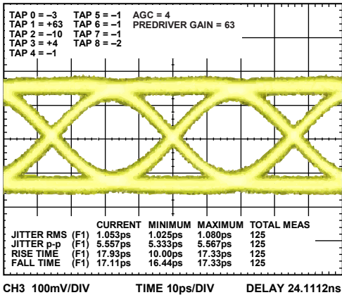
Figure 24. Typical Output Waveform at 28 Gbps, PRBS 2^{31} - 1 Input Data
