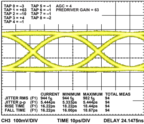
Figure 23. Typical Output Waveform at 22 Gbps, PRBS 2^{31} - 1 Input Data, Input Signal = 300 mV p-p Differential
