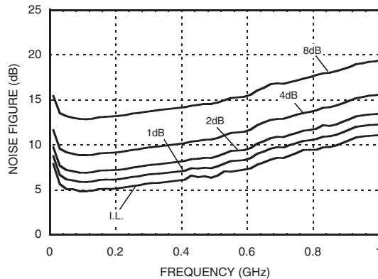
Noise Figure vs. Attenuation State
