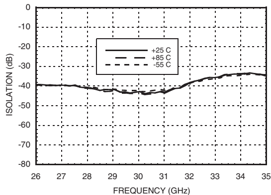
Reverse Isolation vs. Frequency Over Temperature, 5V @ 800mA
