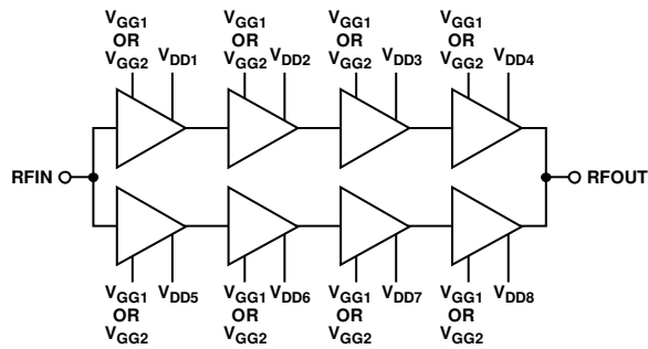
Figure 34. Simplified Functional Block Diagram
