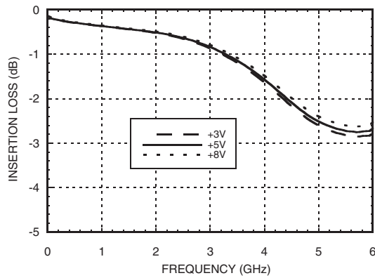
Insertion Loss vs. Vdd
