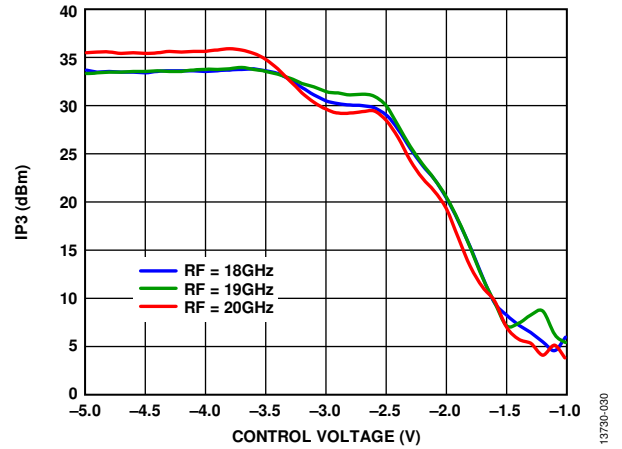
Figure 30. Output IP3 vs. Control Voltage at Various RF Frequencies, LO = 4 dBm
