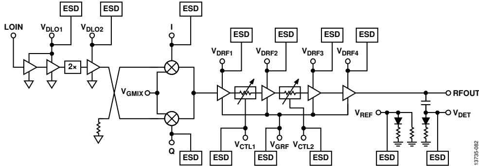
Figure 82. Upconverter Circuit Architecture
