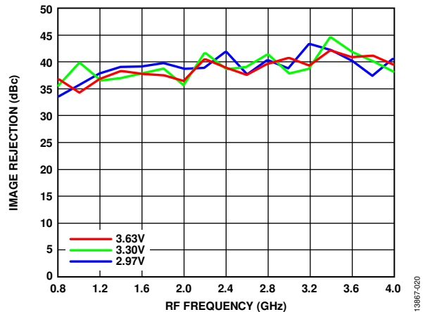
Figure 20. Image vs. RF Frequency at Various V_{CCdr} , 56 MHz Filter
