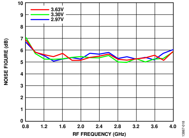
Figure 18. Noise Figure vs. RF Frequency at Various V_{CCdr} , 56 MHz Filter
