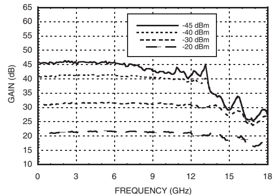
Response vs. Input Power [1][3][5]
