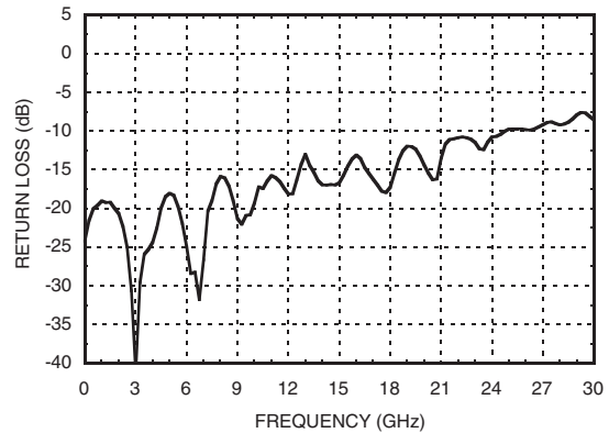
Clock Input Return Loss [1][2][3][4]
