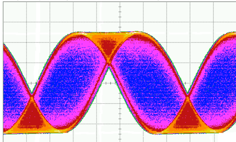
Output Eye Diagram Continuous Snapshot for 15 GHz Input Signal
